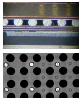
Reliability(X-RAY / Cross Section)
