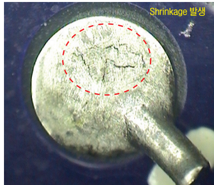
Traditional Sn3Ag0.5Cu Joint
