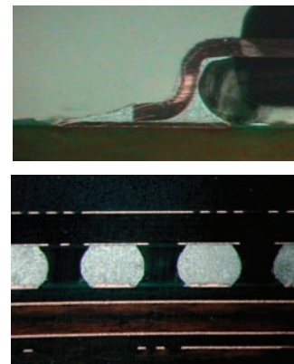
Reliability(Cross Section)
